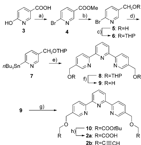
Scheme 1. Synthesis of the decorated terpyridine motifs: a) i: POBr 3 , 170 °C, ii: MeOH, 90 %; b) NaBH 4 , EtOH, 87 %; c) DHP, PTSA, CHCl 3 , 81 %; d) n BuLi, THF, −78 °C, ( n Bu) 3 SnCl, 75 %; e) 2,6-dibromopyridine, [Pd(PPh 3 ) 4 ], toluene, 54 %; f) HCl, MeOH, 64 %; g) for 10 : tert -butyl bromoacetate, aq NaOH 50 %, TBAB, CH 2 Cl 2 , 48 %; for 2b propargyl bromide, aq NaOH 50 %, TBAB, CH 2 Cl 2 , 85 %; h) 25 % TFA in CH 2 Cl 2 , 85 %.
